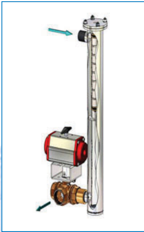
MAGNETIC CORE IN PURGE MODE
